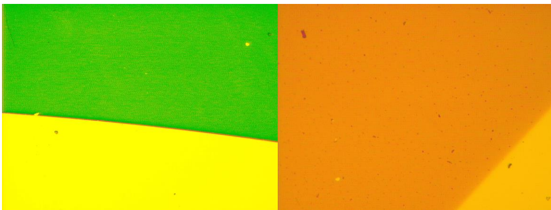
[Figure 4.3] 80nm sample (left) 40nm sample (right) of MoO 3 both masked using silicon clamped to the substrates surface.
