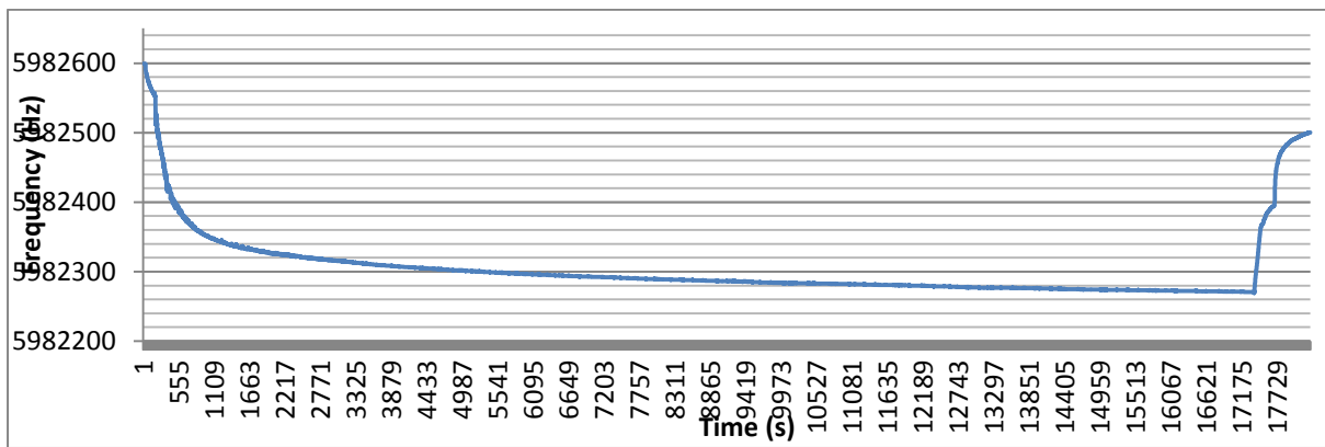
Figure [4.9] 50nm deposited thin film of MoO 3 frequency response after exposure and reapplication of vacuum.
