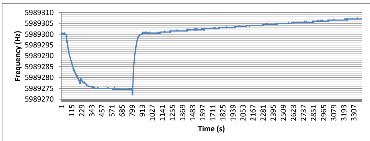
Figure [4.7] Clean Quartz Monitor Crystal frequency response during exposure to environment and reapplication of vacuum.
