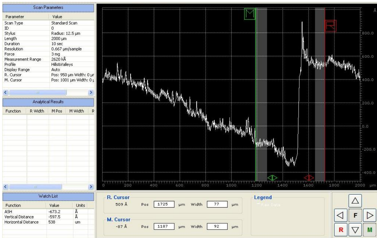
[Figure 4.5] Screenshot of height verification using Dektak stylus profiler of 60nm MoO 3 deposited film immediately after deposition
