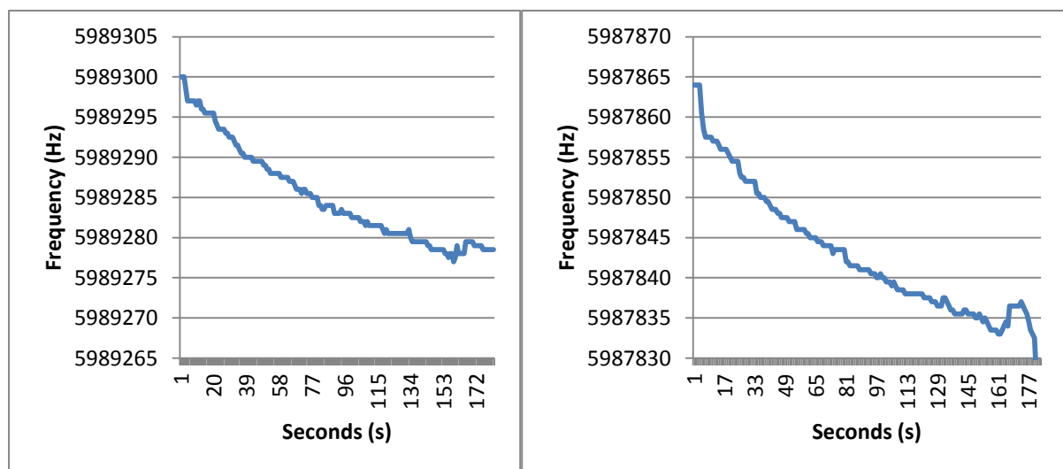
Figure [5.2.1]: Comparison of nitrogen venting for clean crystal (Left) and crystal deposited with 10nm MoO 3 (Right).
