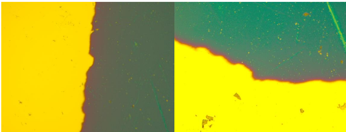
[Figure 4.2]. Two images of 60nm MoO 3 deposited onto silicon substrates shielded using a clamp.
