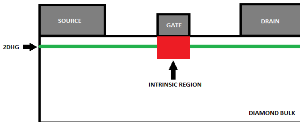
Figure [3]. Demonstrates the operation of a simple FET constructed using a surface doping technique to provide a 2DHG to form under the diamond substrates surface. Under the gate remains intrinsic diamond.
