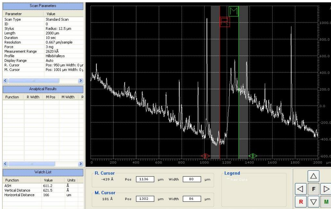
[Figure 4.6] Screenshot of height verification using Dektak stylus profiler of 60nm MoO 3 deposited film after exposure. Note the large spikes which are assumed to be particles resting on the surface.
