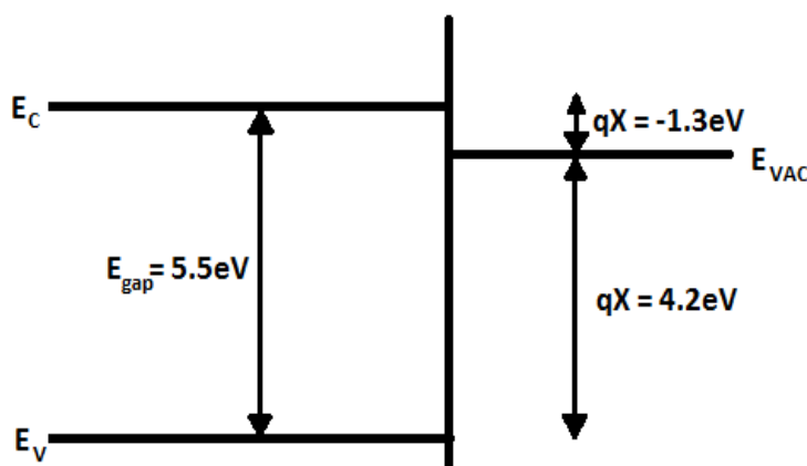
Figure [1] – Band diagram structure for energy of interface between diamond (left) and hydrogen termination (right).
