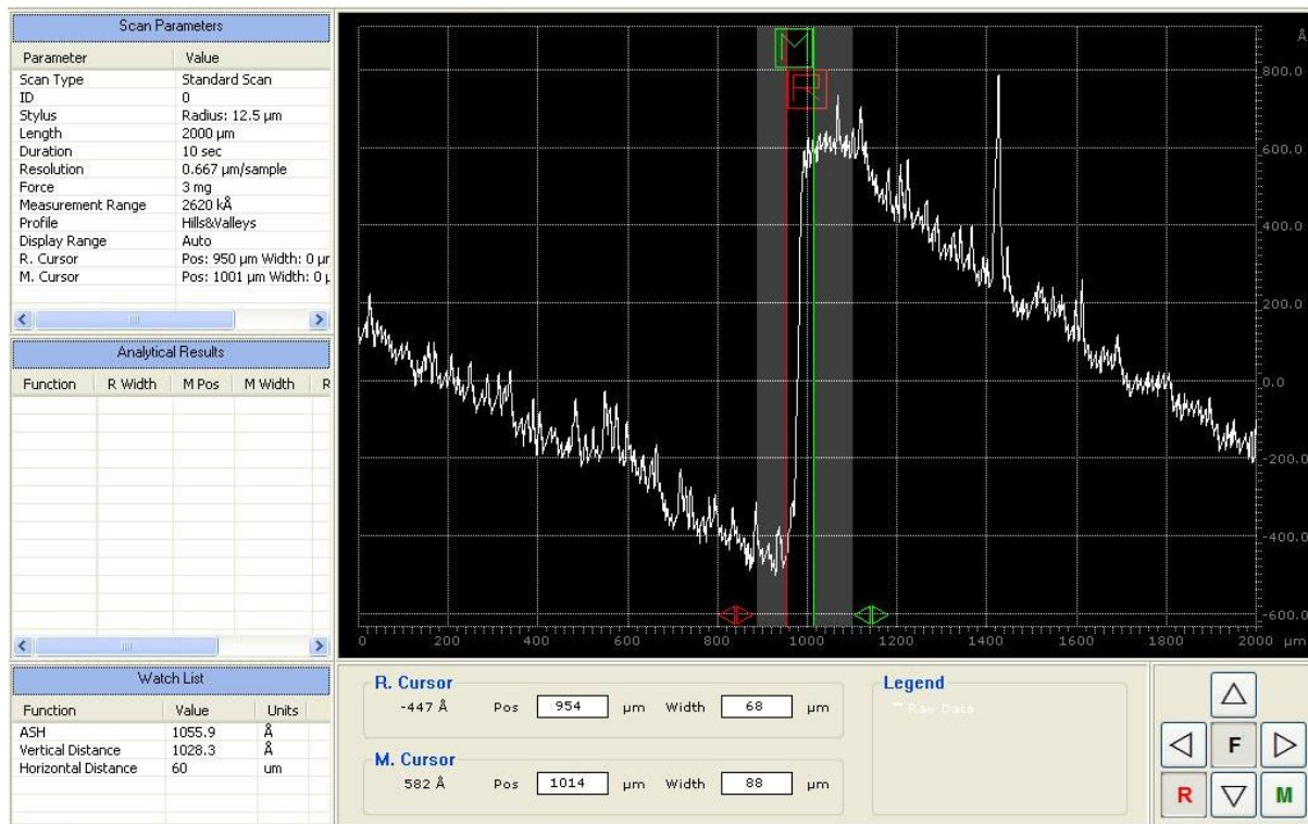
Figure [4.4] Screenshot of height verification using Dektak stylus profiler of 100nm MoO 3 deposited film immediately after deposition. Note the majority consistency of the surfaces.
