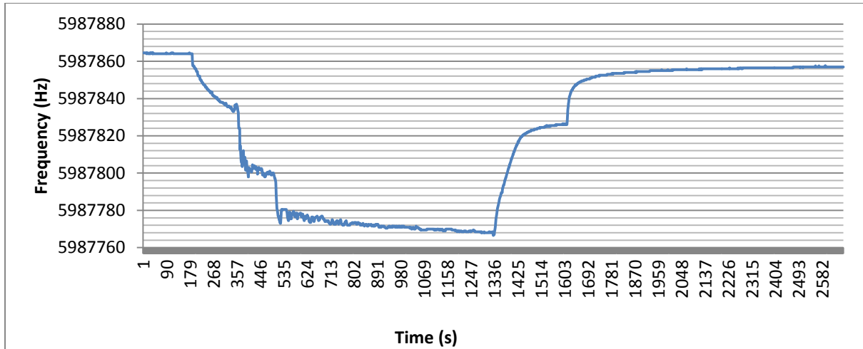
Figure [4.8] 10nm deposited thin film of MoO 3 on clean crystal frequency response after exposure and reapplication of vacuum.
