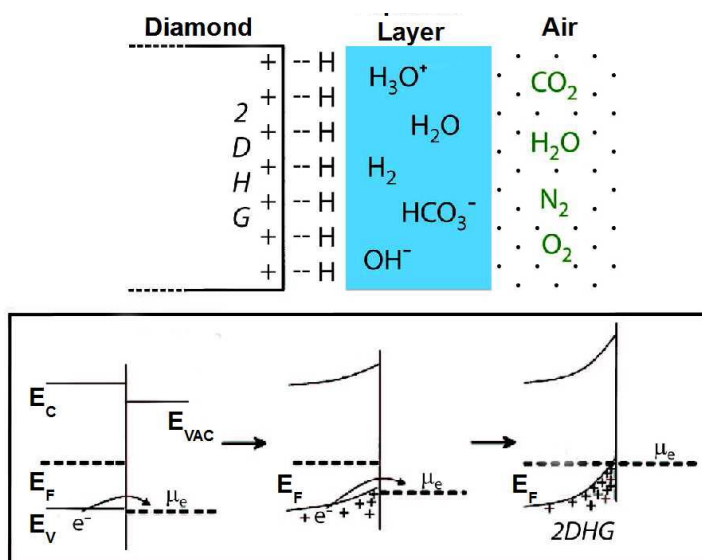
Figure [2] – Diagram showing aqueous region at hydrogen terminated diamond surface and transfer of charge resulting in electron deficient channel forming a 2 dimensional hole gas (2DHG) below the diamonds surface. Taken from “High Performance Hydrogen-terminated diamond field effect transistors, Stephen A. O Russell 2013”
